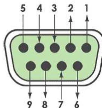
DB9 Female
