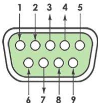
DB9 Male
